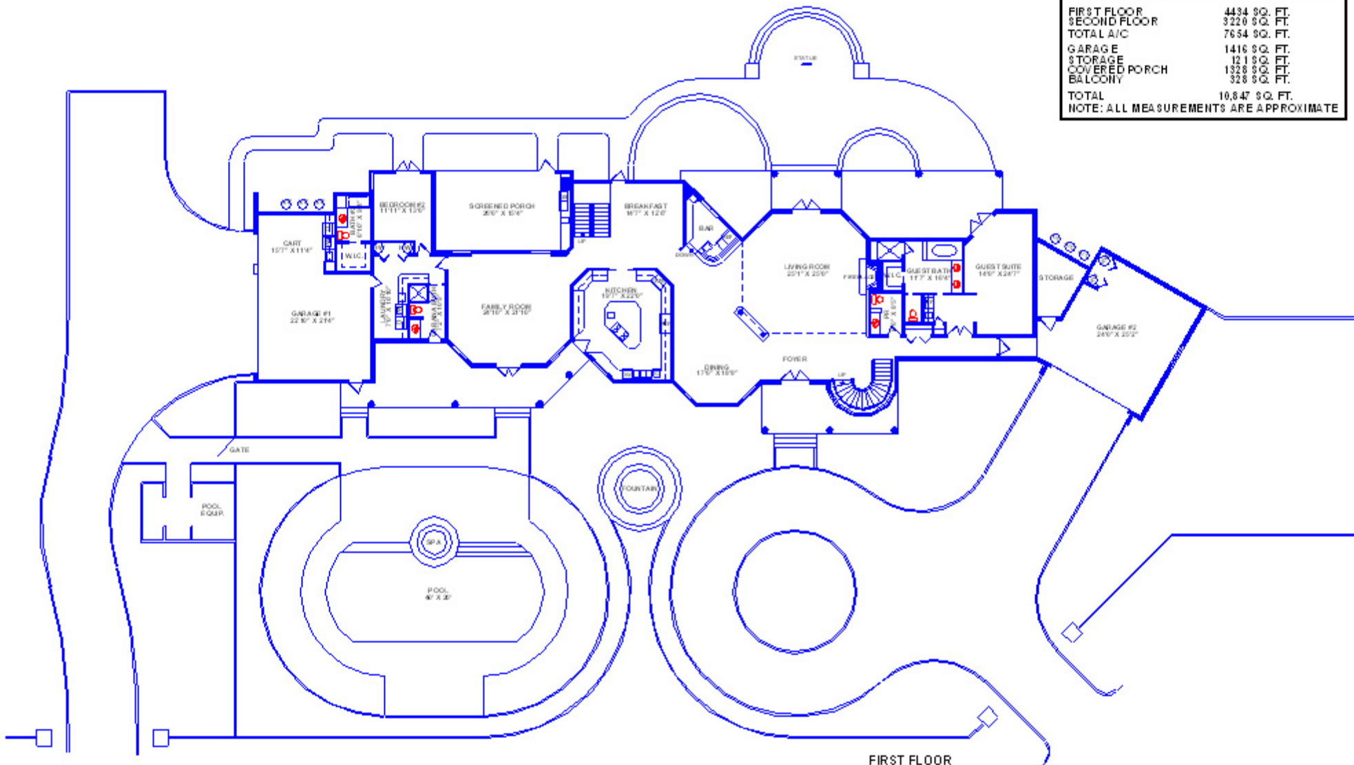
FIRST FLOOR
